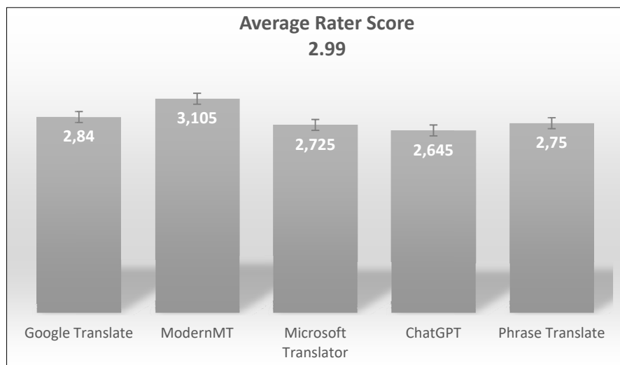
Figure 1. Rater Scores
