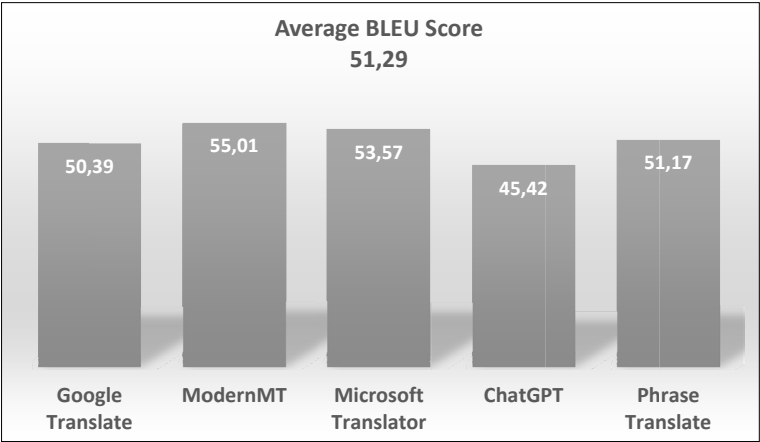
Figure 2. BLEU Scores
